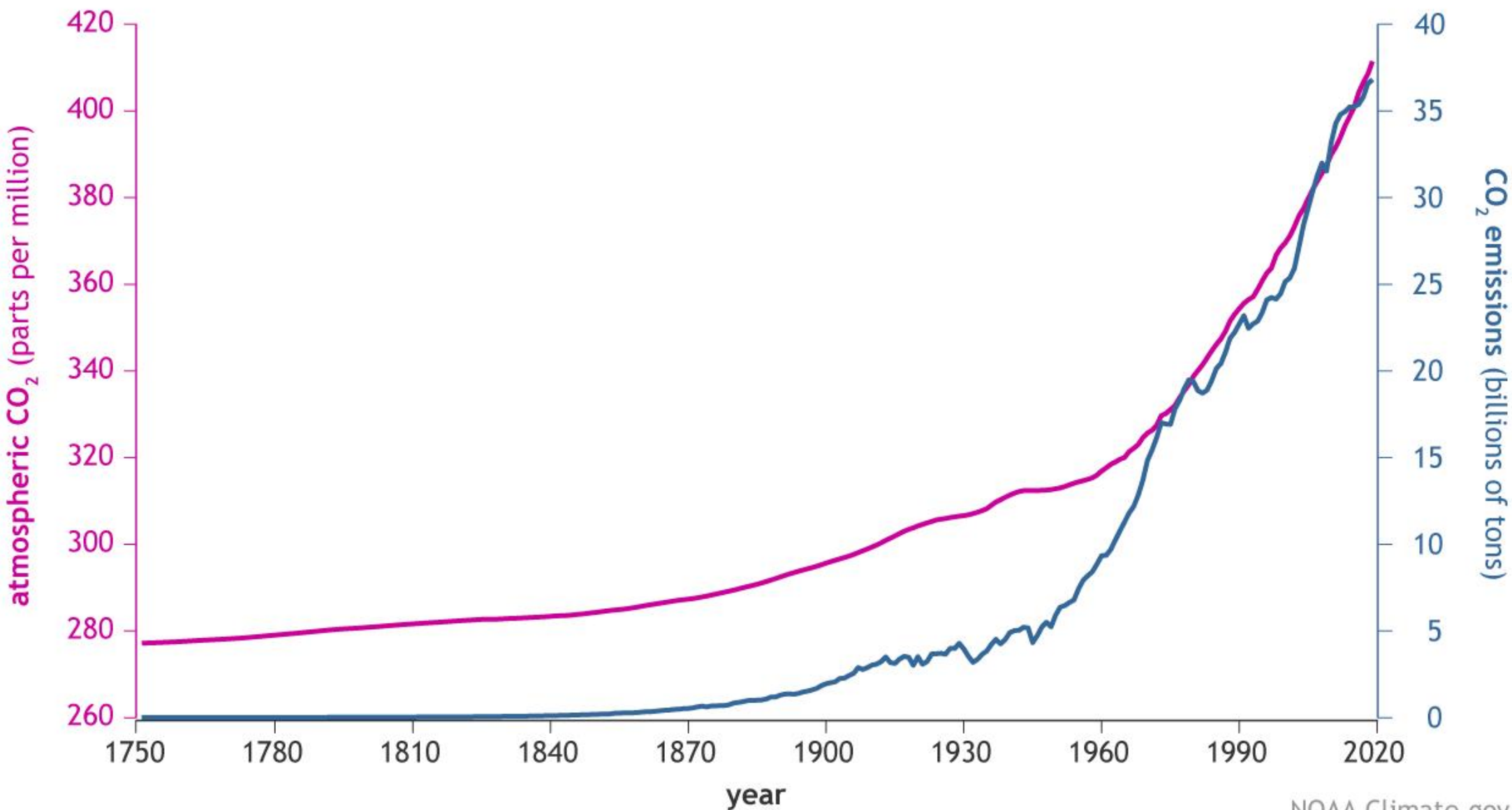
CO 2 in the atmosphere and annual emissions (1750-2019)
